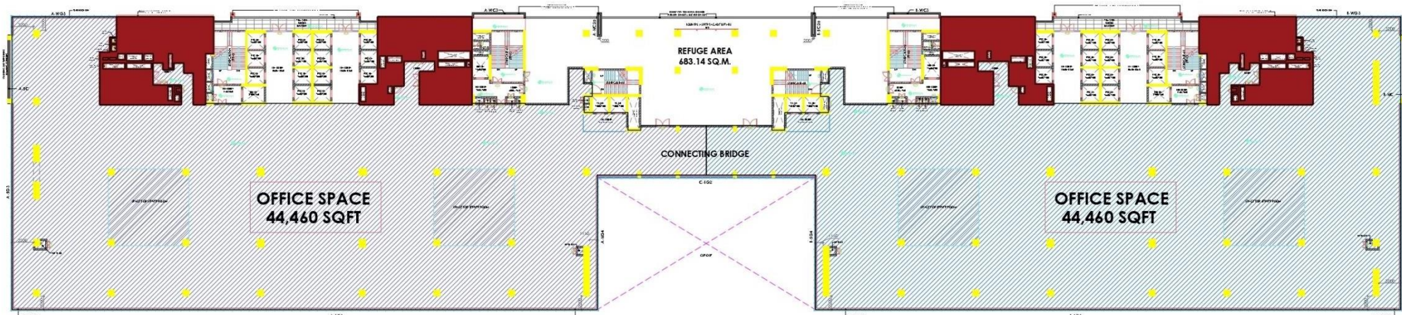
TWELFTH FLOOR PLAN
